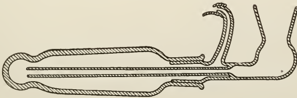
FIG. 7.—Centrifugal elutriator bottle; longitudinal section. (From U. S. Dept. of Agr., Bureau of Soils Bul. 24.)
