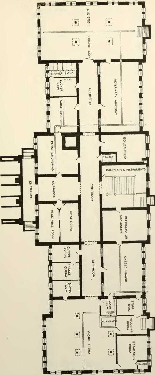
BASEMENT PLAN, AGRICULTURAL HALL, NORTH CAROLINA COLLEGE OF AGRICULTURE AND MECHANIC ARTS.
