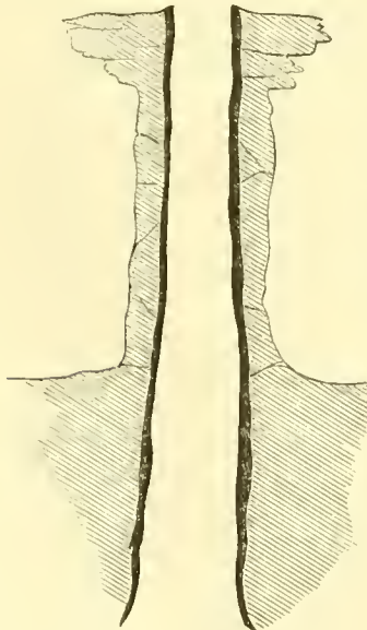
Fig. 43. Tree-casts in a lava stream.
