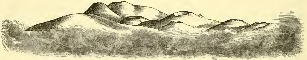
Fig. 33. The Summit of Hualalalā seen from Mauna Lōa (9000 feet).
