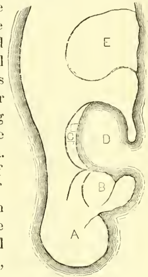
Fig. 14. Plan of the Kōko Craters. A, smooth grassy summit; B, small crater; C, spring of fresh water; D, deep crater open to the sea; E, large dry crater broken down towards the sea.
