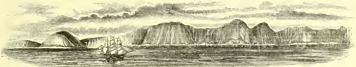
Fig. 5. Eastern end of Oahu. From the north, distant fifteen miles.
