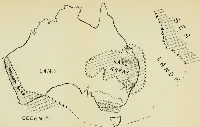
Fig 8. Triassic Distribution of Land and Sea
