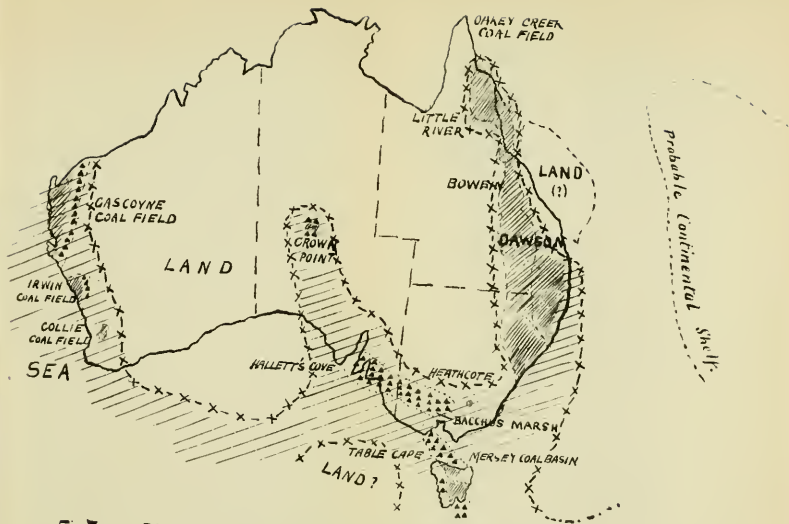
Fig 7. PERMOCARB s Distribution of Land & Sea.
