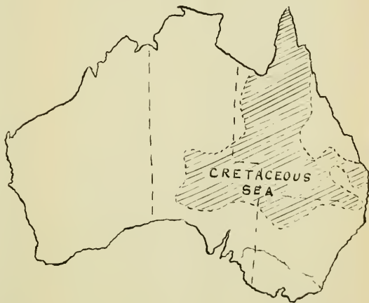
Fig 9. Distribution of Land and Sea in the Cretaceous. The Marine Area is Shaded.
