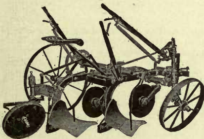
2259. Riding gang-plow.
