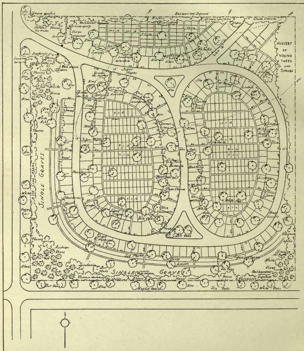
2103. Ground plan of a landscape cemetery.
