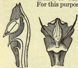
2650. The pendent anther in Caelogyne speciosa .
