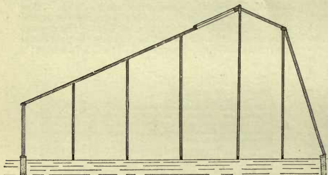
2148. Showing type of greenhouse constructed to obtain the maximum amount of light in short winter days. Modification of type shown in Fig. 2147. Obstructs more light than Fig. 2147, but could be built wider.
