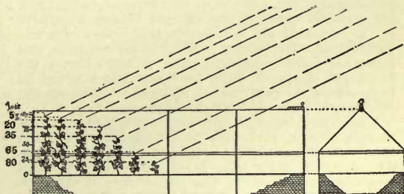
2144. Showing longitudinal and cross sections of a greenhouse with partitions running north and south, and illustrating the effect of poor light conditions. The oblique lines represent the path of the sun's rays.
