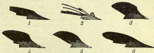
2251. Types of moldboard plows adapted to different kinds of plowing: 1, prairie breaker bottom; 2, rod breaker bottom; 3, stubble bottom; 4, general-purpose bottom; 5, black land bottom; 6, tame sod breaker bottom.
