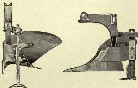
2250. Landside and back view of steel moldboard plow, showing subsoiling attachment.
