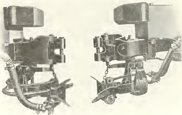
AUTOMATIC COUPLER FOR TRAIN HOSE
