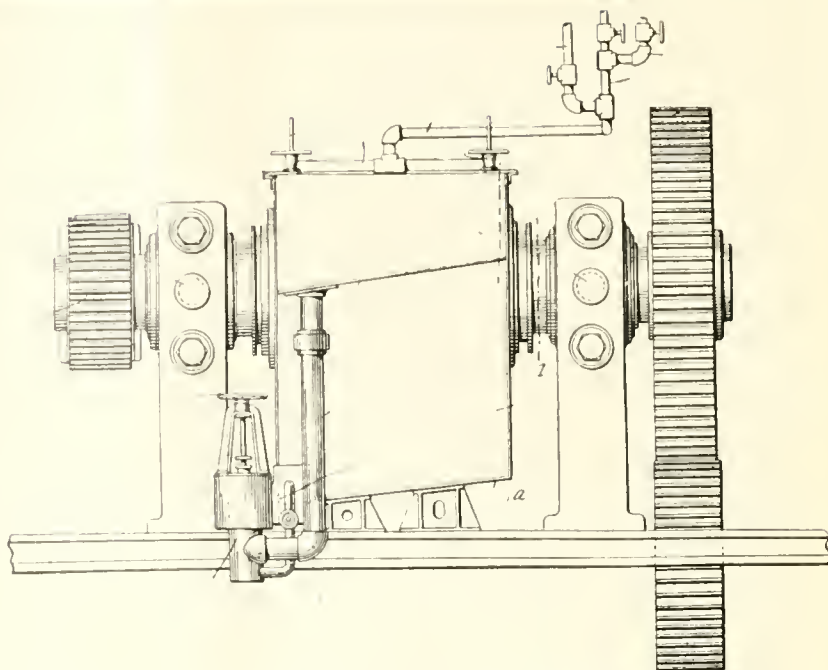
A NEW MACHINE FOR WASHING RUBBER.
