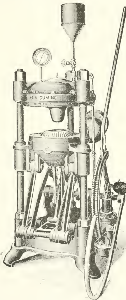
HYDRAULIC HAT PRESS.
