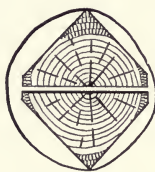
FIG. 72.—Method of sawing triangular ties from tie logs.
