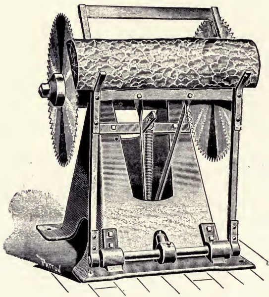
FIG. 29.—The Trevor stave bolt equalizer.
