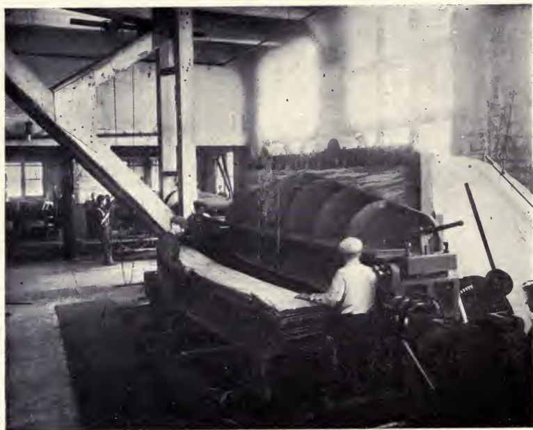
FIG. 19.—A veneer-slicing machine in operation, cutting Circassian walnut veneers. Note the veneer flitch fastened above. This is dropped vertically against a sharp knife. The men are engaged in piling the sliced veneers as they emerge at the base of the machine.
