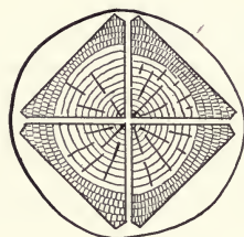
FIG. 72.—Method of sawing triangular ties from tie logs.
