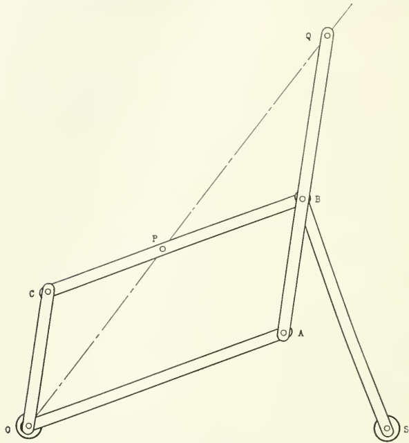
FIG. 5. PANTAGRAPH.
