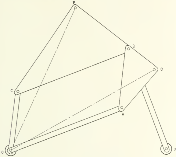
FIG. 6. PLAGIOGRAPH.
