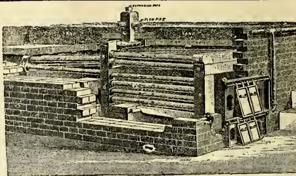
"CHILWELL NURSERIES" HORIZONTAL TUBULAR BOILER.
