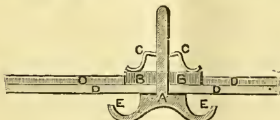
FIG. 98.—NEWTON'S METHOD OF ROOF-GLAZING.
