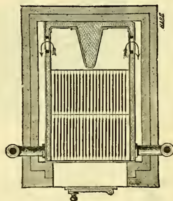
SECTIONAL PLAN.
