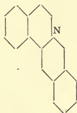
Berberine
