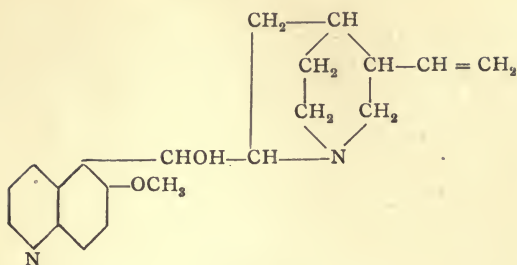
Quinine
