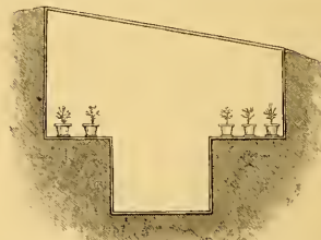
Fig. 2.—Section of Earth Pit with Sunk Walk.
