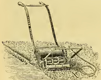
1 MONARCH MS. CHAIN OFF SET FOR CUTTING TURF.
