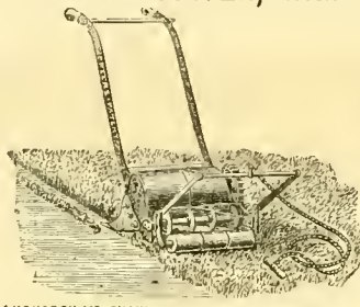
1 MONARCH M. CHAIN OFF SET FOR CUTTING TURF.
