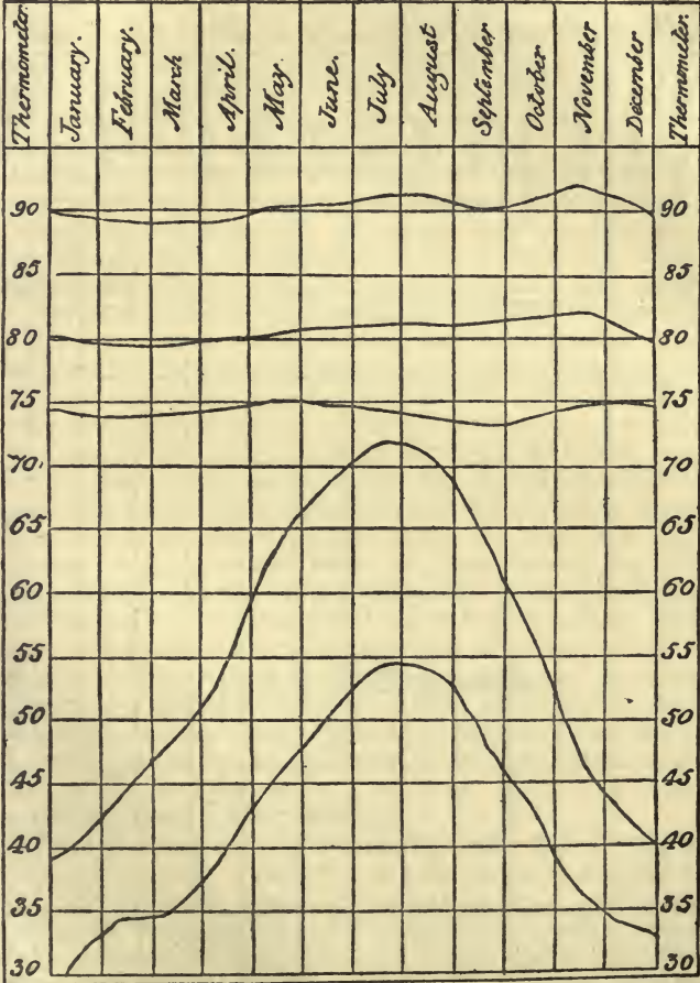
The three upper curves show the Means of the highest, lowest, and mean temperatures at Pará for four years. The two lower curves show the highest and lowest monthly mean temperatures at London.
