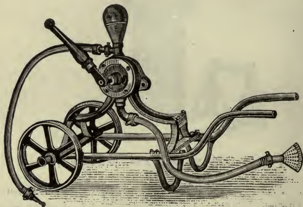
FIG. 49.—SEMI-ROTARY WING PUMP.
