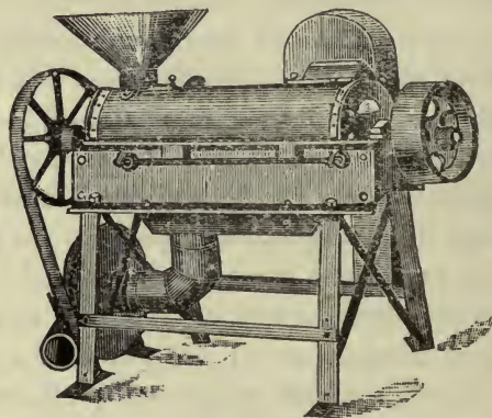
FIG. 58.—THE COFFEE HULLER.
