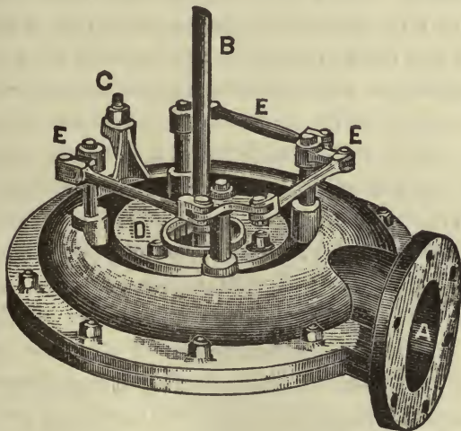
FIG. 11.—THE TURBINE.
