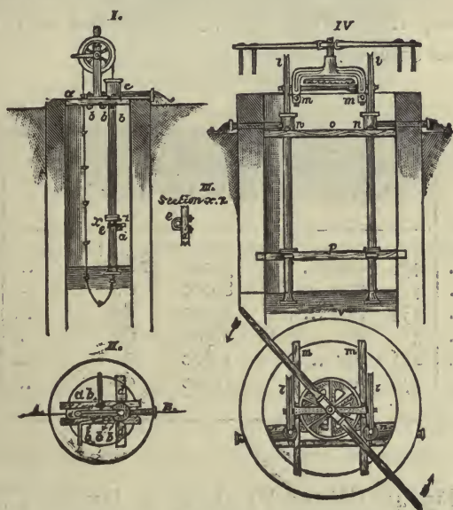
BULLOCK-POWER LIFT.
