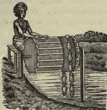
FIG. 43.—PERSIAN WHEEL (RATNAGIRI TYPE).
