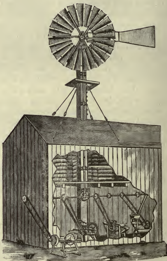
FIG. 7.—THE AEROMOTOR (POWER-MILL).
