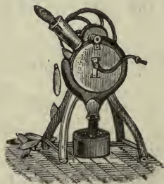
FIG. 51.—MAIZE-HULLER.
