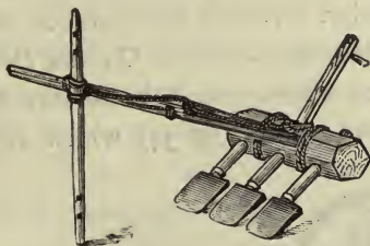
FIG. 32.—MADRAS BULLOCK-HOE.
