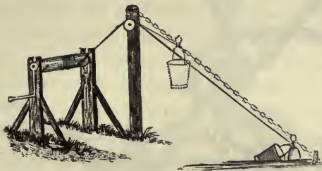
FIG. 48.—WINDLASS AND BUCKET LIFT.
