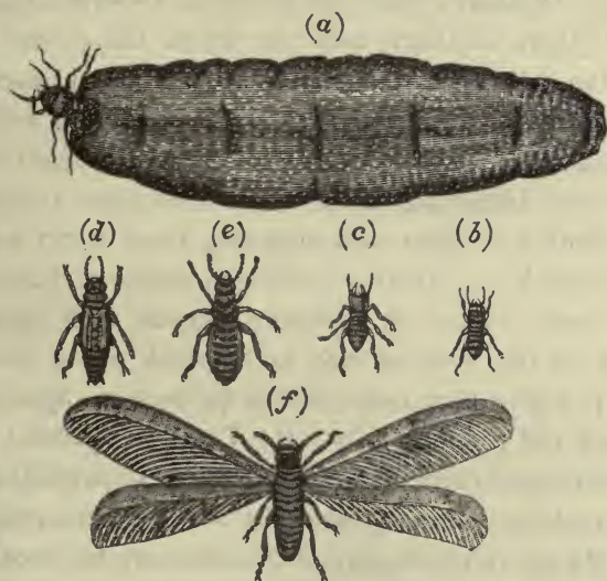
FIG. 73.—THE WHITE-ANT.
