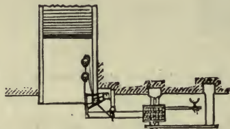
FIG. 38.—THE DOUBLE-MÔT (SECTION THROUGH AB.).
