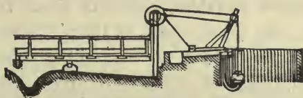
FIG. 40.—SUBBA RAO'S WATER-LIFT (SECTION).
