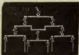
FIG. 20.—SWINGLE FOR THREE ANIMALS.
