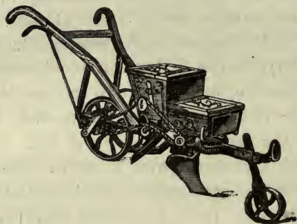
FIG. 30.—HENDERSON CORN PLANTER AND FERTILIZER DISTRIBUTOR.
