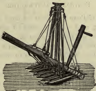
FIG. 29.—MADRAS TINED SEED-DRILL.
