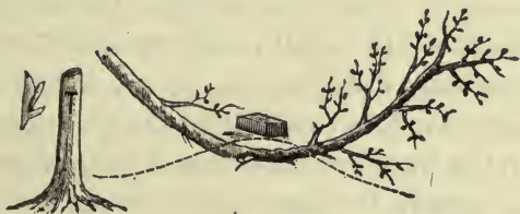
FIG. 60.—BUDDING.
