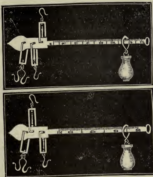
FIG. 53.—STEEL-YARD FOR WEIGHING 15 TO 50 lbs. (FIG. 52 REVERSED).
