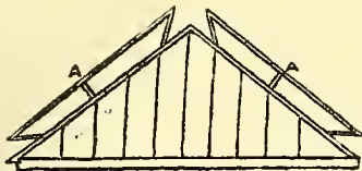
Fig. 1 shows the east end, one sash on the south side, and one on the north side, being tilted. A A are two chucks, which tilt the sashes. The sashes are hinged on the other side.
