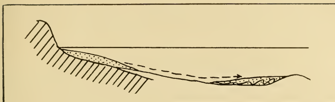
Fig. 3. Diagram illustrating Hahn's hypothesis of submarine slumping
