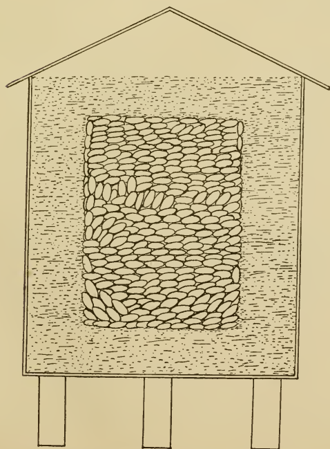
Fig. 2.—Section through Bakhari , as used in Bihar, to show how the grain is stored with Bhusa (Chaff) all around it.
