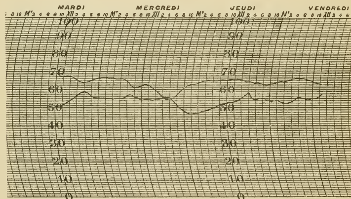
Relationship between lint-weight and atmospheric humidity. Upper curve, humidity ; lower curve, lint-weight.
