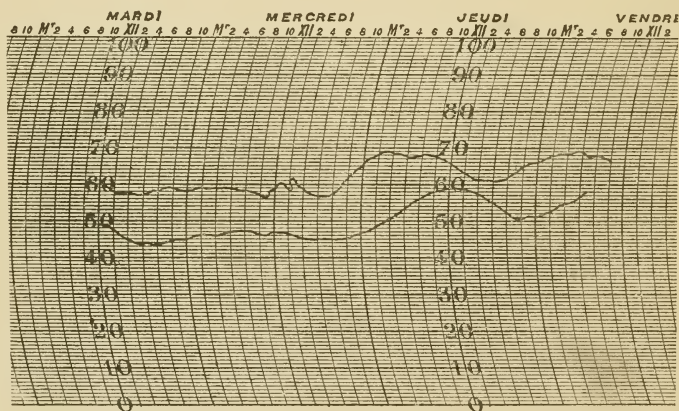
Relationship between seed-weight and atmospheric humidity. Upper curve (1), humidity ; lower curve (2), seed-weight.
