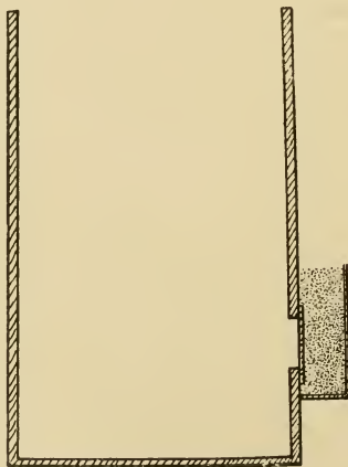
Fig. 2.—How openings, if desired at the lower parts of bins for taking out the stored grain, may be protected with sand.
