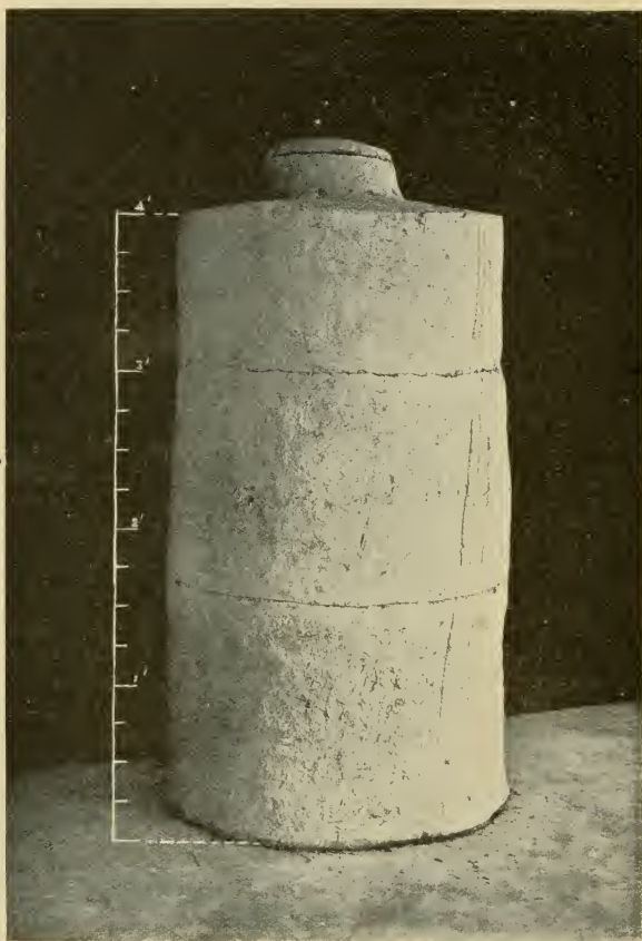
Storage receptacle ( Kothi ) made, in three pieces, of unburnt clay. Inside measurements, 4 feet high and 2 feet in diameter.
