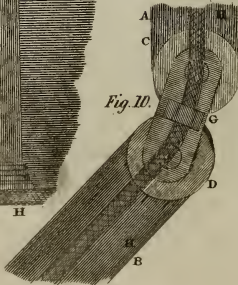
M r Furness's Air Tight Door Hinge.
