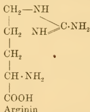
Arginin
