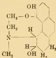
Morphin
