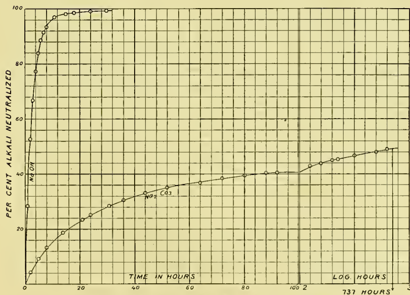
FIG. I.—HYDROLYSIS OF METHYL SALICYLATE.
