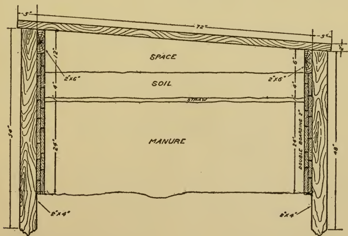
Fig. 13.—Section of a hotbed frame with details of measurements. Reproduced from a Cornell bulletin.
