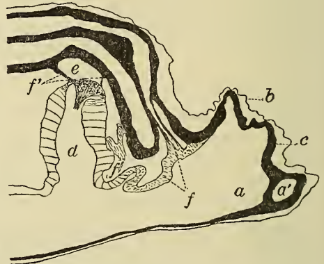
FIG. 6. A drawing, from camera lucida outlines, of part of an oblique, transverse section through a contracted polyp of Cornularia minuta . a , the point of junction of the body cavity and one of the stolons; a' , an oblique section through one of the endodermal canals of the stolon; b , the perisarc; c , the wall of the polyp, represented in black; d , the stomodæum; e , the siphonoglyphe; f and f' , mesenteries. \times 65.5 .
