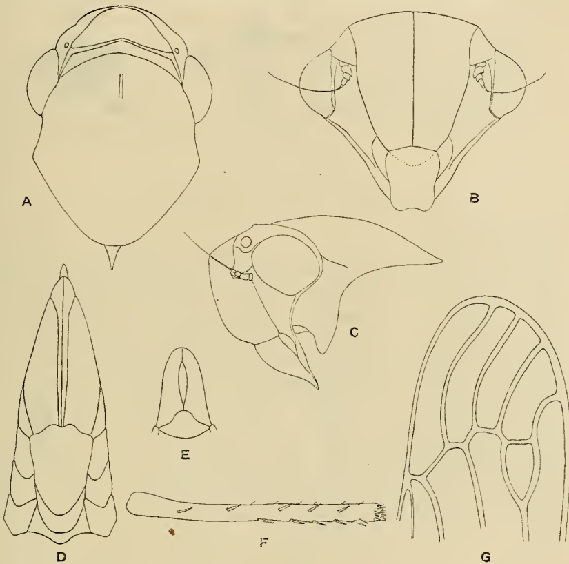
FIG. 3. Signoretia tagalica sp. nov. a, upper surface of head, pronotum, scutellum; b, face; c, side view of head and pronotum; d, female genitalia; e, male genitalia; f, posterior tibia; g, apical portion of tegmina.
