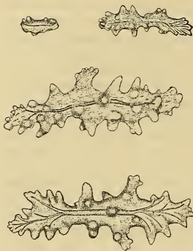
FIG. 2. Spicules from the stem cortex of Lithophytum rigidum sp. nov. \times 112.5 .
