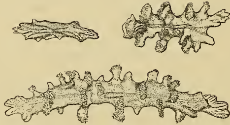
FIG. 1. Spicules from the stem cortex of Lithophytum philippinensis sp. nov. \times 112.5 .
