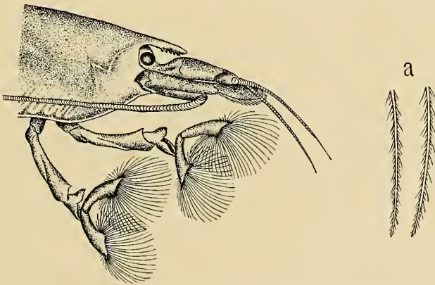
Fig. 3. Atya molluccensis de Haan. A female. a, hairs on chelipeds, enlarged.
