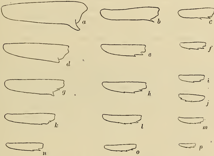
FIG. 1. Atya molluccensis de Haan. a, b, c , specimen 1, meri of the right third, fourth, and fifth legs, respectively; d, e, f , specimen 2, meri of the right third, fourth, and fifth legs, respectively; g, h, i , specimen 3, meri of the right third, fourth, and fifth legs, respectively; j , specimen 3, merus of the left fifth leg; k, l, m , specimen 4, meri of the right third, fourth, and fifth legs, respectively; n, o, p , specimen 5, meri of the right third, fourth, and fifth legs, respectively.
