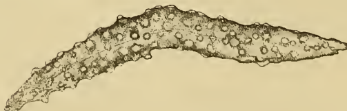
FIG. 3. A spindle from the canal wall of Lithophytum rigidum sp. nov. \times 47.3 .
