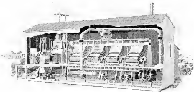
FIG. 155. — SECTION THROUGH A GINNEY. Showing four gins, press, suction pipe, and shafting.
