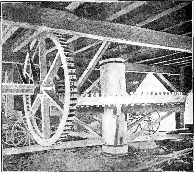
FIG. 164.—THE PROPELLING MECHANISM OF AN OLD HORSE-POWER GIN. Showing large wheels with wooden cogs. (By permission of D. A. Tompkins.)
