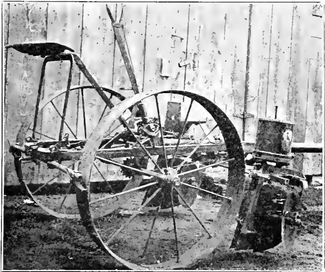
FIG. 55.—CHECK-ROW CORN PLANTER, WITH DOUBLE DISKS TO OPEN A DEEP FURROW.
