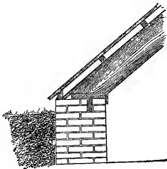
243. The sill and roof construction.
