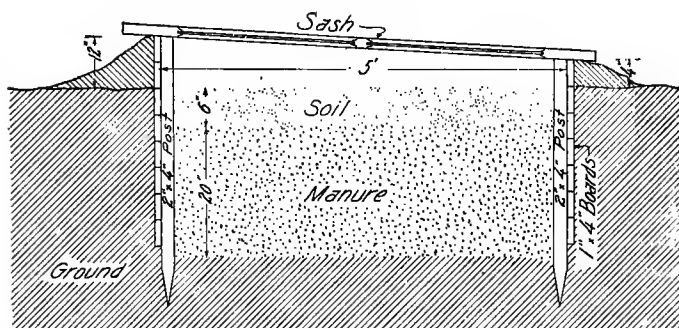
216. A manure-heated hotbed.
