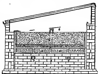
218. Pipe-heated hotbed.
