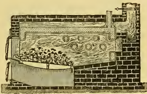
Check-end Saddle Boiler, simple and durable.
