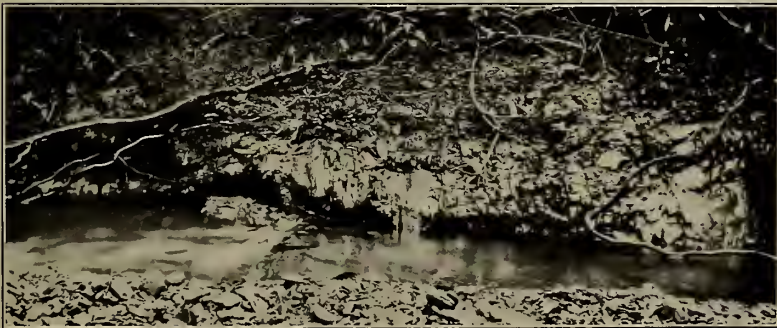
Fig. 3. Nearly vertical Vigo shale.
