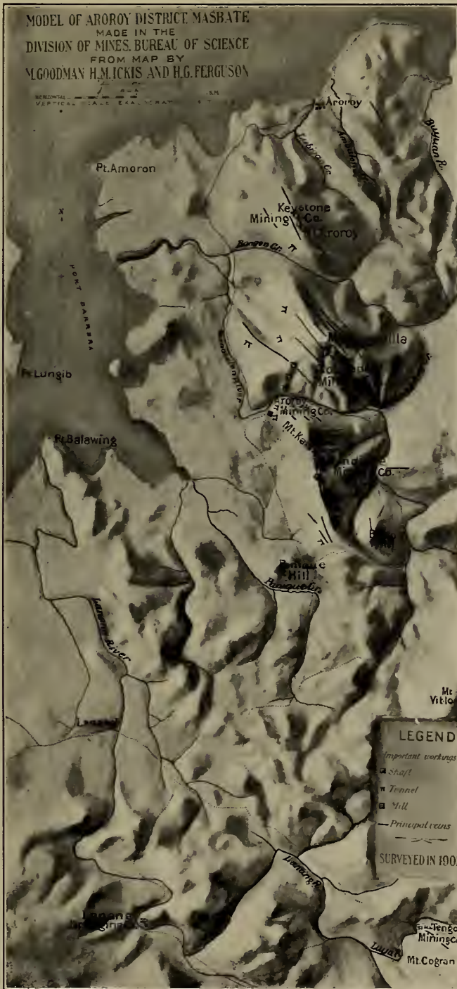
PLATE III. RELIEF MAP OF ARORÓY DISTRICT.
