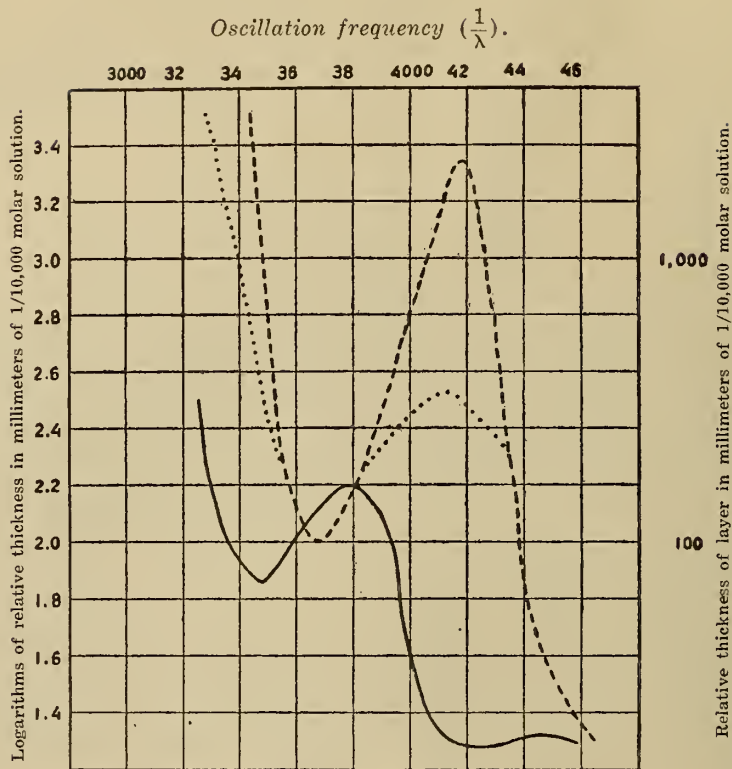
FIG. 1.—Dash curve=phenol.
