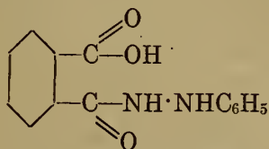
Anilidophthalamic acid.
