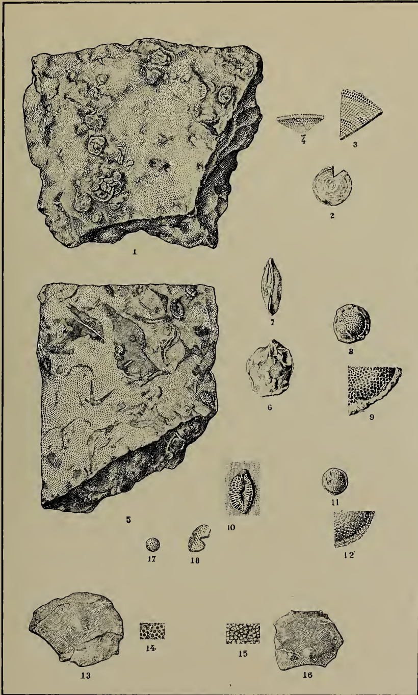
Fig. 1. Operculina costata d'Orbigny. 2. Orbitolites complanata Lam. 3, 4. Sections of the same much enlarged. 5. Orbitoidal and coralline limestone. 6, 7. Lepidocyclina insulæ-natalis Jones et Chap., central part. 8. Lepidocyclina formosa Schlm. (?) 9. Lepidocyclina formosa Schlm. (?), detail of the surface, much enlarged. 10. Flabellum sp. 11, 12. Lepidocyclina formosa Schlm. (?) 13-16. Lepidocyclina insulæ-natalis Jones et Chap. 17, 18. Portions of radiolarian tests.
