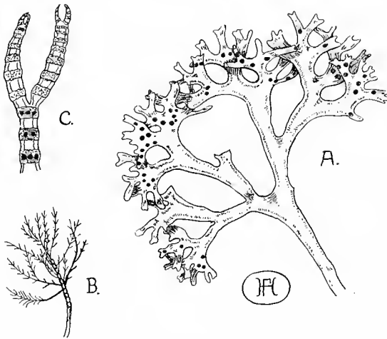
FIG. III.—Red Algæ. A, Carrageen ( Chondrus crispus ), the dark patches being due to groups of carpospores (p. 228). B, Corallina . C, Apex of a branch of Ceramium (after Kützing), with groups of tetraspores (shown black).
