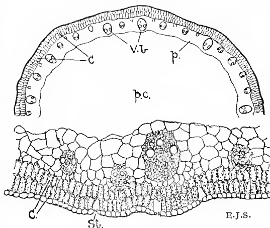
FIG. 86.—Transverse section of the leaf of the Jointed Rush ( Juncus articulatus ). The upper figure shows a diagram of about half the section, the lower a small segment on a larger scale. C., assimilatory tissue; p., parenchyma; p.c., central cavity; St., stoma; V.b., vascular bundles.
