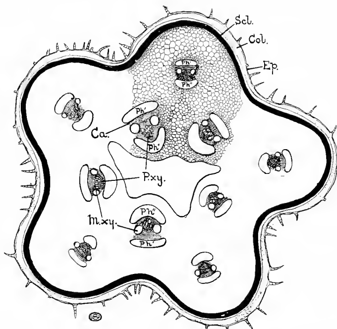
FIG. 37.—Diagram of a transverse section of the stem of the Vegetable Marrow ( Cucurbita ). Ca. , cambium; Col. , collenchyma; Ep. , epidermis; M.xy. , metaxylem; Ph. ', outer phloem; Ph. "', inner phloem; P.xy. , protoxylem; Scl. , sclerenchyma (black).
