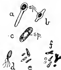
FIG. 145.— a-c , spore-formation in Bacteria. a , Bacillus tetani ; b , Bacillus of malignant oedema; c , Bacillus cedamitis . d-f , nitrogen-fixing Bacteria. d , Azotobacter ; e , Clostridium pasteurianum sp.; f , Bacillus radiculicola . (After Engler and Prantl, and Ellis.)
