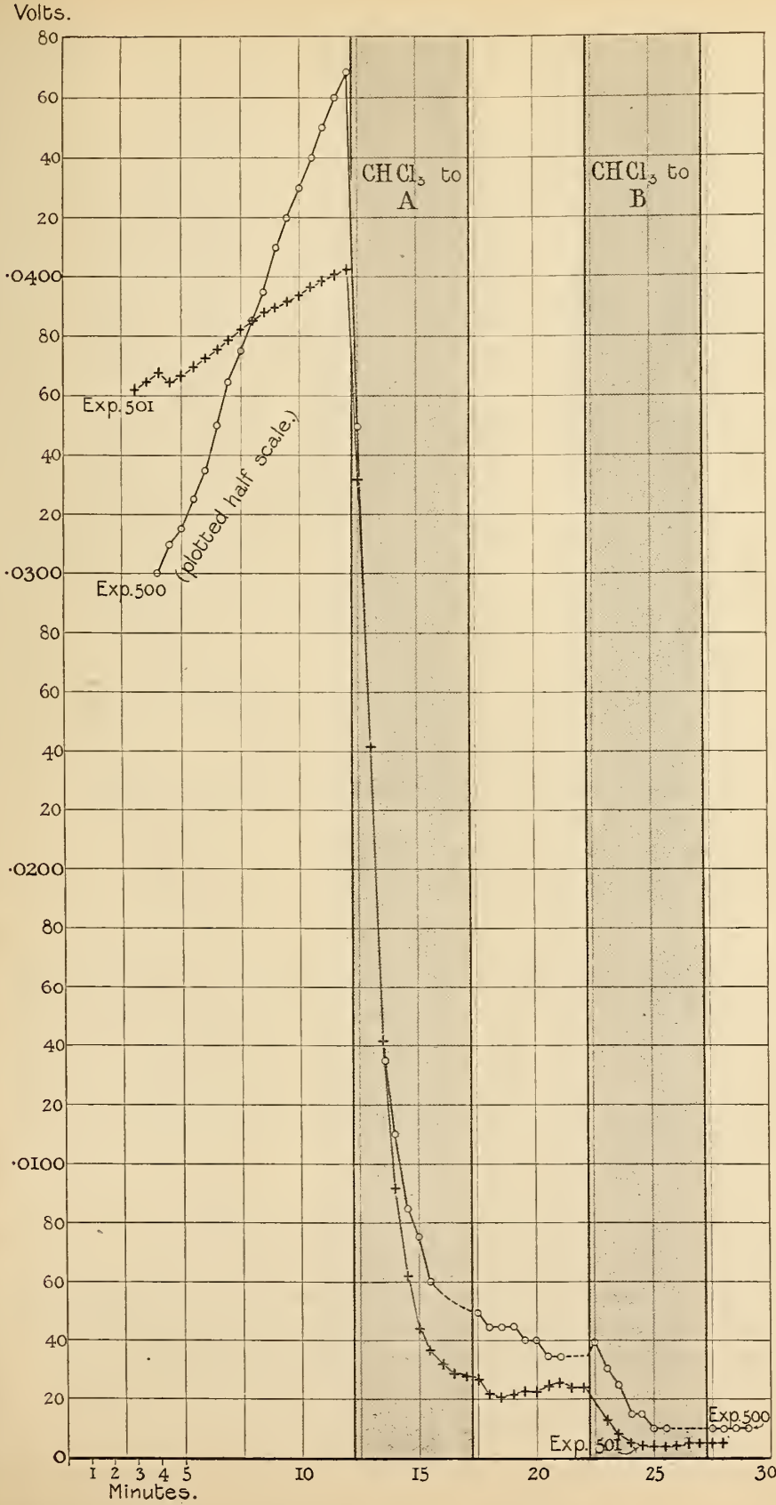
FIG. 3.—Series I. \text{CHCl}_3 (16 per cent.) to Parts of Skin. A = Outer Surface to Electrodes; B = Inner Surface. Experiment 501, \text{CHCl}_3 for 5-minute intervals; Experiment 500 for 3.5-minute intervals.
