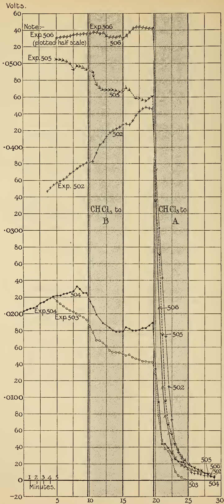
FIG. 2.—Series I. \text{CHCl}_3 (at approximately 16 per cent.) applied at the shaded parts. A = Outer Surface of Skin to Electrode ; B = Inner Surface to Electrode.
