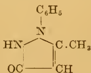
Phenyl-1-methyl-5-pyrazolon-3
