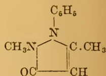
Phenyl-1-dimethyl-2,5-pyrazolon-3 (Isoantipyridin)
