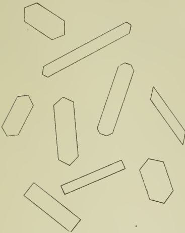
FIG. 52.—Phytosterol crystals.
