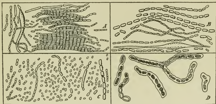
FIG. 83.—Vinegar organisms. A, Bacterium (Mycoderma) aceti ; B, Bacterium pasteurianus ; C, Bacterium küzingianum ; D, B. pasteurianum , showing the mucilaginous sheath. This mucilaginous material causes the cells to stick together in large masses, forming the so-called "mother of vinegar."—(Marshall.)
