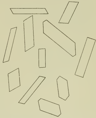
FIG. 53.—Cholesterol crystals.
