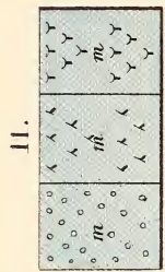
Melaphyrites.
