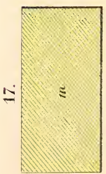
Marms primitives.
