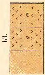
Argiles primitives.
