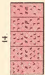
Serpentinites.
