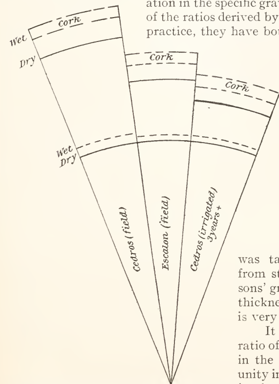
FIG. 17.—Relative thickness of cortex in stems of irrigated and field plants, the wood cylinders being of equal diameter when dry.
