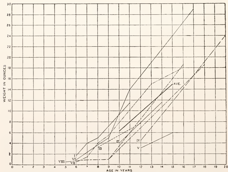
FIG. 15.—Upper diagram: Curves correlating age and height of plants in table 39. Lower diagram: Age and weight correlated. The same plants.
