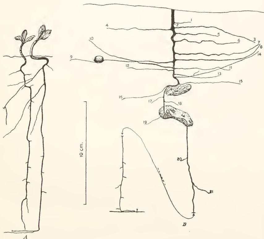
FIG. 19.—A, the roots of two seedlings grown in 4-square-inch paper tubes; B, a root-system of about the same age, growing in a box. \times 9/20 .
