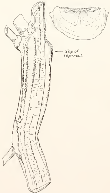
FIG. 18.—A successful sectorial root-stem cutting, showing complete healing.
