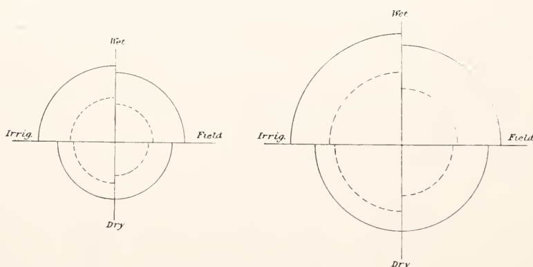
FIG. 16.—Relative dimensions of wood cylinder and cortex, wet and dry, in twigs of field and irrigated plants. \times 20 .
