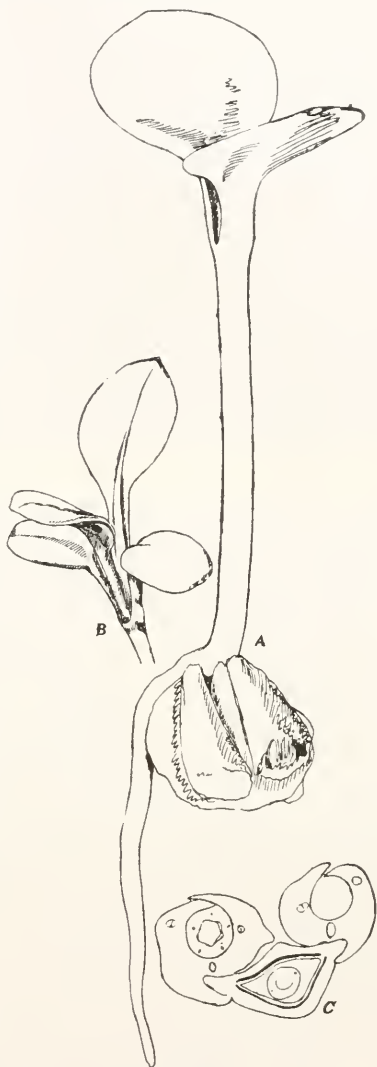
FIG. 8.—A, a fully germinated seedling of guayule, before induration, \times 8 ; B, cotyledons and first two foliage leaves; C, transverse section through achene of a ray flower and its two attached disk flowers.
