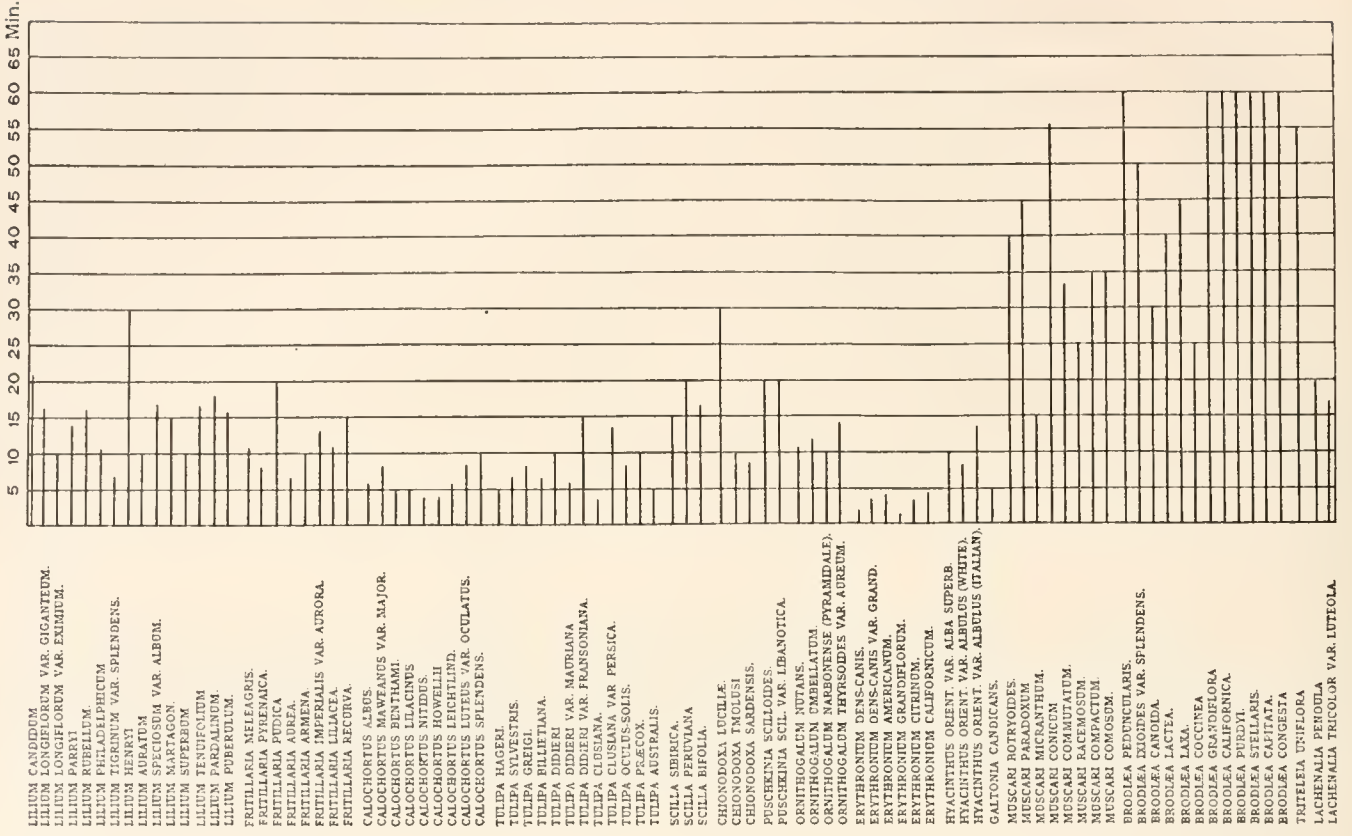
CHART I.—The Ferric Chloride Reactions of Various Starches.
