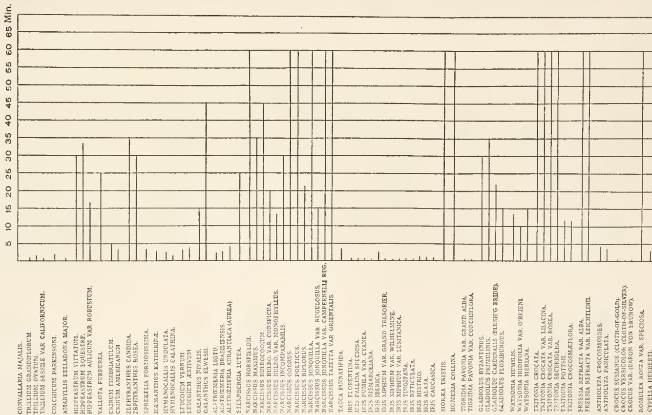
CHART H.—The Pyrogallic Acid Reactions of Various Starches—continued.
