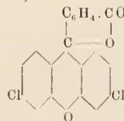
Fluoresceinchlorid (farblos).
