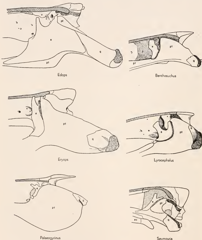
Fig. 5. Comparative external views of left palato-quadrate complex of various labyrinthodonts; diagrammatic, and freely restored. Presumed structures and areas in cartilage, stippled. Cross-hatching refers to bone sectioned. Data for figures 5 to 8 have been derived as follows: Edops after Romer and Witter; Eryops after Sawin; Benthosuchus after Bystrow; Lyrocephalus after Sive-Söderbergh, partly based on Aphancramma and Trematosaurus ; Palaeogyrinus after Watson; Seymouria after White.
