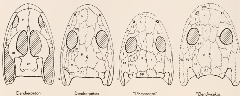
Fig. 21. Dendrerpetonts from the Joggins. After Steen.
