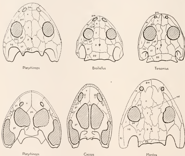
Fig. 29. Eryopsoids: dissorophids and Mordex . Platyrrhinops , Mordex after Steen; Broiliellus , Cacops after Williston.
