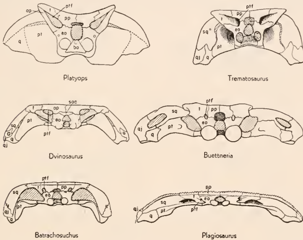
Fig. 3. Posterior views of skulls. Platyops after Efremov; Trematosaurus after Jaekel; Dvinosaurus after Bystrow; Buettneria after Case, Wilson; Batrachosuchus after Watson; Plagiosaurus after Huene.
