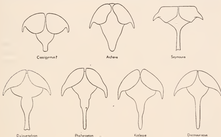
Fig. 14. Diagrams of dermal shoulder girdles of various anthracosaurs. Crassigyrinus (?) after Huxley; Seymouria after White; Diplovertebron , Phaiherpeton after Fritsch; Kotlassia after Bystrow; Discosauriscus after Credner.
