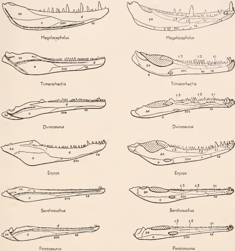
Fig. 10. Lower jaws (continued). Megalocephalus after Watson; Trimerorhachis after Case; Dvinosaurus after Bystrow; Eryops after Sawin; Benthosuchus after Bystrow; Parotosaurus composite.
