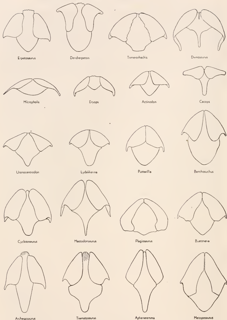
Fig. 13. Diagrams of dermal shoulder girdles (clavicles and interclavicle) of various temnospondyls, seen in ventral view. Dendrerpeton , after Steen; Trimerorhachis , Buettneria after Case; Dvinosaurus , Benthosuchus after Byströw; Micropholis , Lydekkerina after Watson; Actinodon after Gaudry; Cacops after Williston; Uranocentrodon , Putterillia after Broom; Cyclotosaurus , Mastodontosaurus , Metoposaurus after Fraas; Plagiosaurus after Huene; Archegosaurus after Jaekel; Trematosaurus after Burmeister; Aphaneramma after Nilsson.
