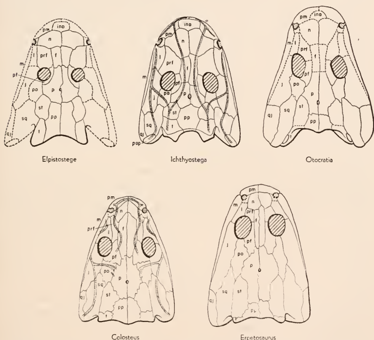
Fig. 15. Skull roofs of ichthyostegals. Elpistostege restored after Westoll; Ichthyostega after Säve-Söderbergh, Westoll; Otocratia after Watson.
