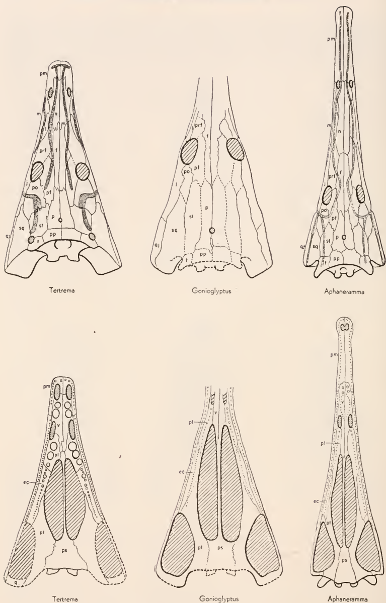
Fig. 33. Trematosaurs. Tertrema after Wiman, Säve-Söderbergh; Gonioglyptus after Huene; Aphaneramma after Wiman, Säve-Söderbergh, Bystrow.
