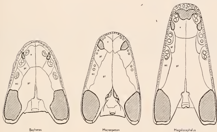
Fig. 19. The palate of loxommids. Baphetes , Megaloccephalus after Watson.
