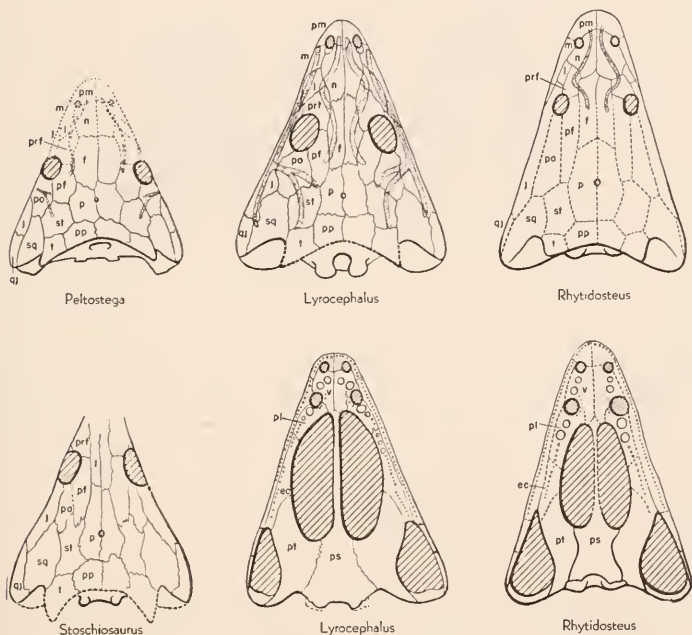
Fig. 34. Trematosaurs. Peltostega , Lyrocephalus after Wiman, Säve-Söderbergh; Rhytidosteus , composite restoration after Owen, Haughton; Stoschiosaurus after Säve-Söderbergh.
