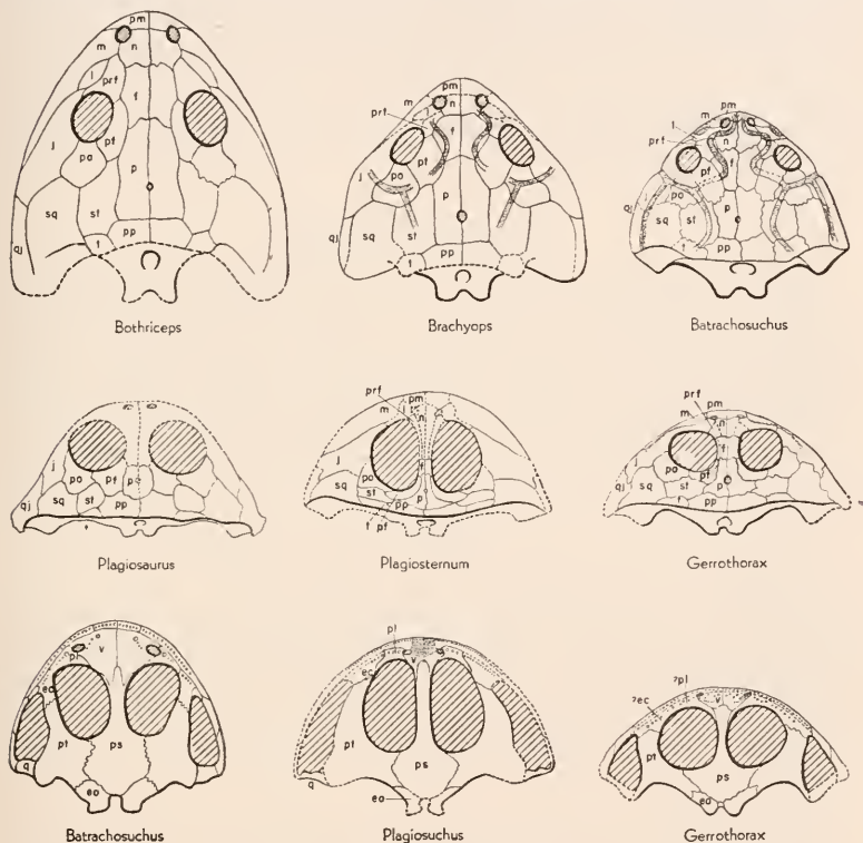
Fig. 40. Short-skulled brachyopoids. Bothriceps , Brachyops after Broom; Batrachosuchus after Watson; Plagiosaurus after Jaekel, Nilsson; Plagiosternum after Fraas, Huene, Nilsson; Gerrothorax after Nilsson; Plagiosuchus after Huene, Nilsson.
