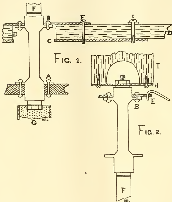
ARRANGEMENT OF BICYCLE HUBS AND ATTACHMENTS FOR ROTATING TABLE
