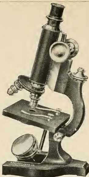
No. 65 B 10mm and 4mm objectives. Double nosepiece. One eyepiece. Cabinet. $35.50 Discount to schools.
