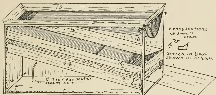
Fig. 6. Collecting machine; B. C. D, three trays; a upper line of the water tank; b iron supports of the box; c parts of the jarring arrangement; d and e cross trays and sections.
