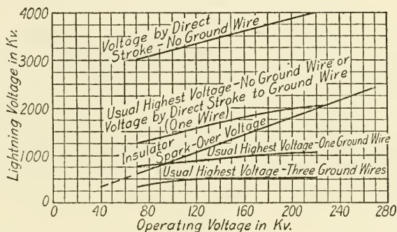
FIG. 22.—Insulator spark-over voltage compared with maximum lightning voltage for severe storms directly over the line
