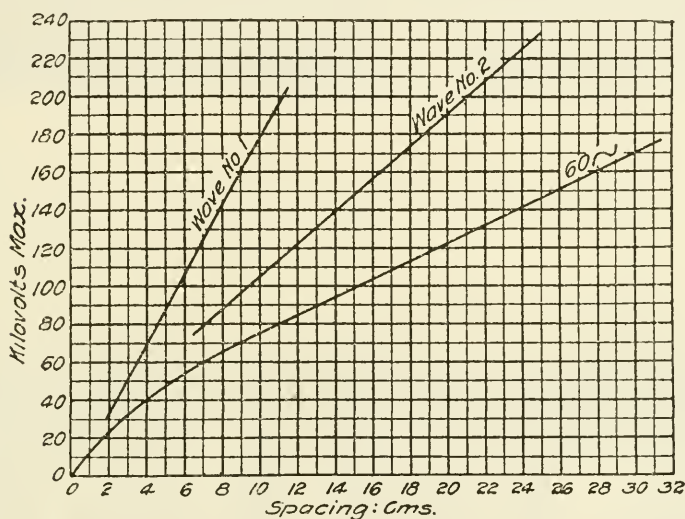
FIG. 26.—Needle-gap spark-over curves for 60 cycles and for impulse waves Nos. 1 and 2. Wave No. 1, single half sine wave impulse; wave No. 2, impulse with steep front, but with a long tail
