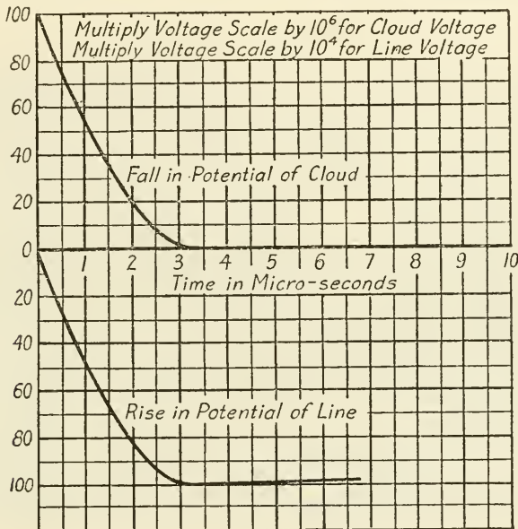
FIG. 16.—Transients for cloud discharge to earth
