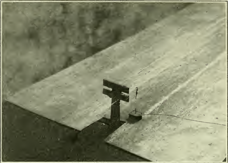
FIG. 19.—SHORT SECTION OF A THREE-PHASE LINE WITH OVERHEAD GROUND WIRE UPON WHICH A STUDY WAS MADE OF INDUCED VOLTAGES BY LIGHTNING
