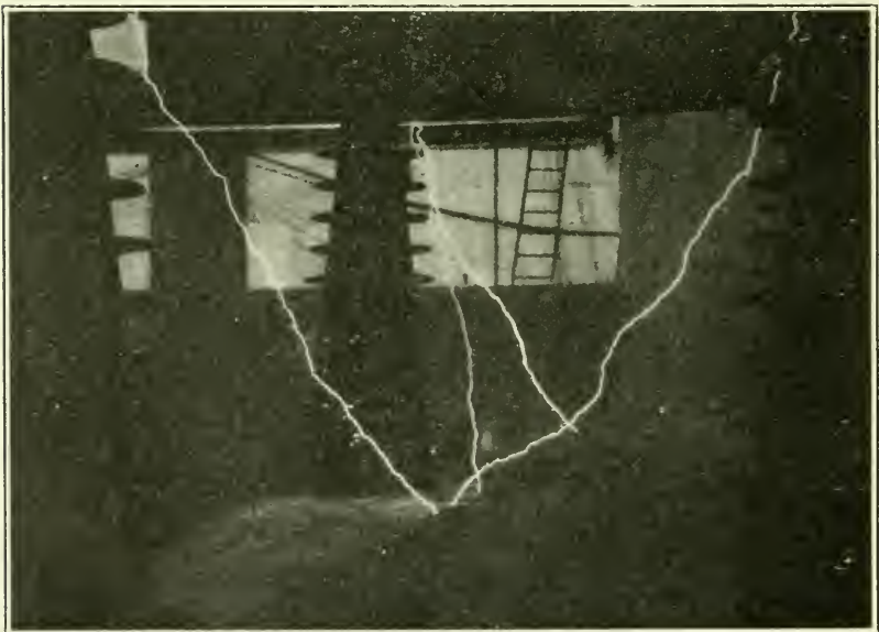
FIG. 20.—LIGHTNING STROKES HITTING THE OVERHEAD GROUND WIRE OF A TRANSMISSION LINE DURING STUDY OF LIGHTNING VOLTAGES INDUCED ON A THREE-PHASE LINE DURING A STORM
