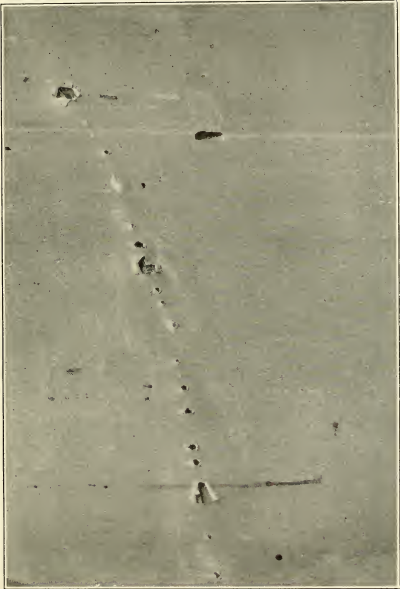
FIG. 9.—METAL "PUNCTURED" BY LIGHTNING
