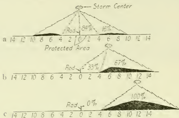
FIG. 35.—Protected area and distribution of hits between a rod and ground for different positions of storm center
