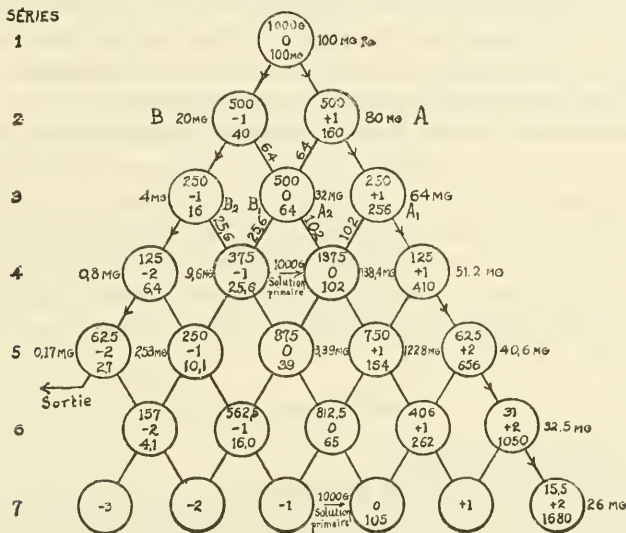
FIG. 1.—The fractional crystallization of radium chloride
