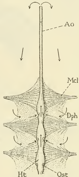
FIG. 26.—Diagram of the typical structure of the heart and diaphragm of an insect, and the course of the circulating blood (indicated by arrows)
