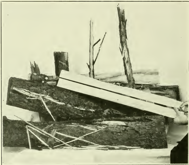
FIG. 8.—WOOD SPLIT BY ARTIFICIAL LIGHTNING
