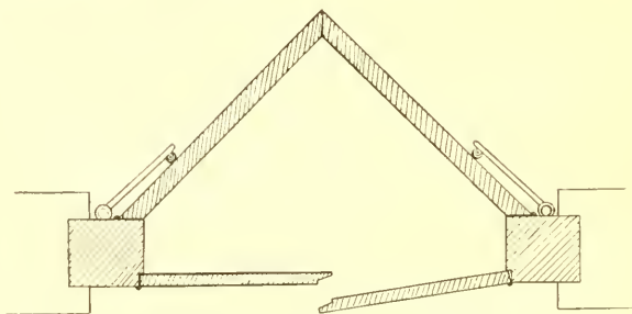
Fig. 2.—Details of double door to Insectary.
