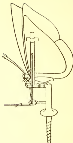
Fig. 2.—Knaggs Butterfly Decoy (side view).
