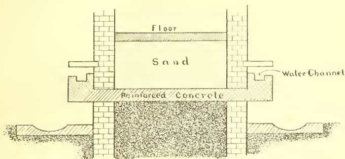
Fig. 1.—Plan for foundation of an Insectary in order to make it ant-proof.
