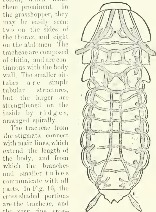
FIG. 16. TRACHEAL SYSTEM.
