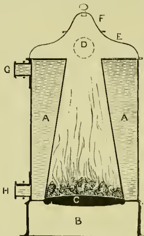
FIG. 260. VERTICAL SECTION OF CYLINDER BOILER.
