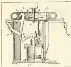
BEAD-RING CLAMPING MACHINE.
