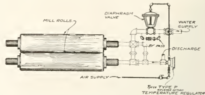
TYPE P TEMPERATURE REGULATING SYSTEM TEMPERATURE IN MILL-ROLLS BY MEANS OF COOLING WATER. NOTE: BY PASS MUST BE CRACKED OPEN TO INSURE CIRCULATION AROUND REGULATOR STEM MILL ROLL TEMPERATURE REGULATOR.
