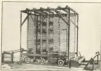
A CORD-FABRIC SPREADER AND DRYER.
