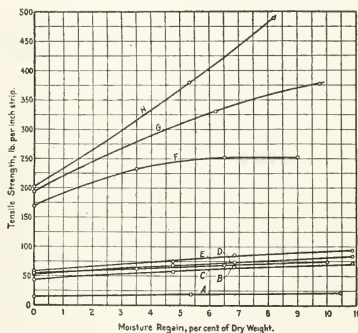
FIG. 1. VARIATION IN TENSILE STRENGTH IN TEXTILES DUE TO MOISTURE.
