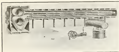
MACHINE FOR VACUUM-DRYING AND SOLVENT RECOVERY.
