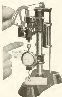
THE WIDNEY RESILIMETER.
