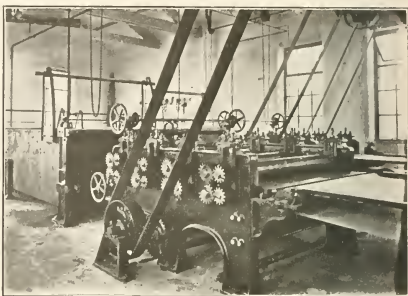
FIG. 2. BELT-STICKING MACHINE.
