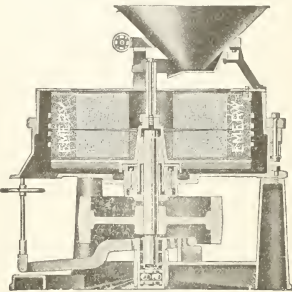
THE STURTEVANT MILL.
