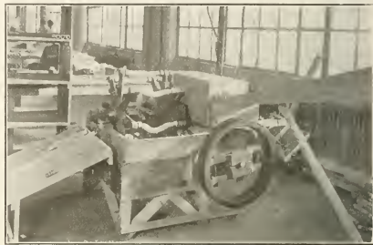
FIG. 10.—PRESSURE LEAKAGE TESTING MACHINE FOR FLEXIBLE HOSE.
