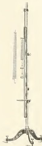
JOLLY SPIRAL BALANCE.
