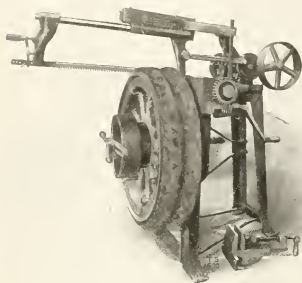
SOLID-TIRE-BASE CUTTING SAW.
