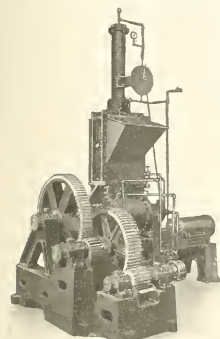
THE BANBURY MIXER.
