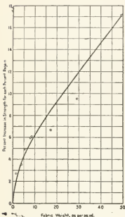
FIG. 2.—RATE OF INCREASE IN TENSILE STRENGTH WITH REGAIN OF FABRIC.
