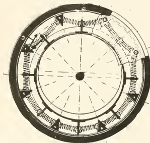
GERMAN SPRING SUSPENSION WHEEL.
