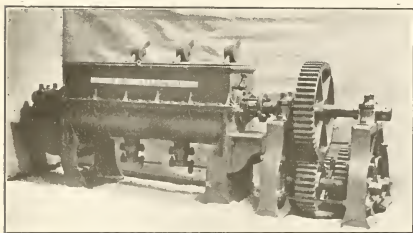
FIG. 1. BALATA-WASHING MACHINE.
