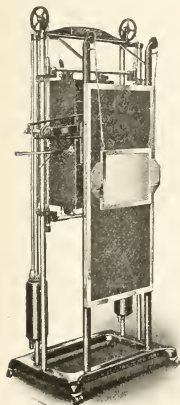
WAPPLER FLUOROSCOPE.
