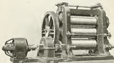
THE W-S-M CALENDER.
