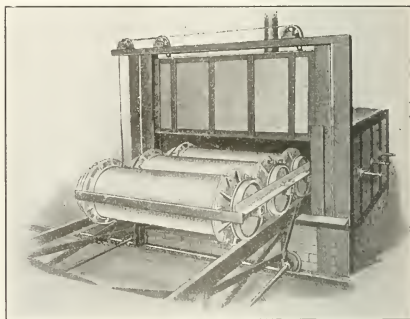
DRUMS CONTAINING TUBE MANDELS BEING ROLLED INTO A SHERARDIZING FURNACE.
