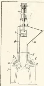
BANBURY MIXER.
