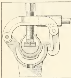
THE "WESTERN" RETREADER.
