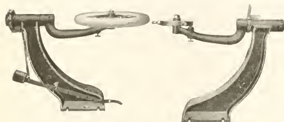
TIRE-BUILDING STANDS. FOOT-OPERATED. HAND-OPERATED.
