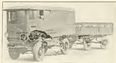
TRUCK AND TRAILER EQUIPPED WITH AIR-BRAKES.
