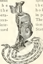
WEED CHAIN JACK.
