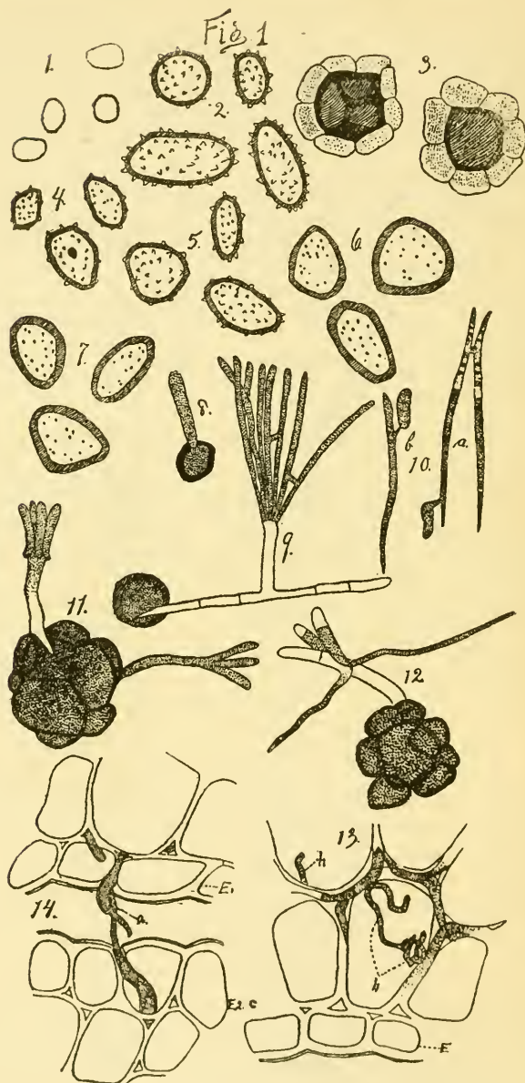
Fig. 57. Smut spores of various kinds. 1. Tall meadow oat smut ( Ustilago perennans ). 2. Timothy smut ( U. striaeformis ). 3. Rye smut ( Urocystis occulta ). 4. Cheat smut ( Ustilago bromivora ). 5. Foxtail smut ( U. neglecta ). 6. Millet smut ( U. panici miliacei ). 7. Sandbur smut ( U. Cusatii ). 8, 9. Tilletia germinating. 10. Secondary spores from conidia. 11, 12. Urocystis spores germinating. 13, 14. Mycelium of same. h . Suckers or haustoria. h . Hyphae passing from one leaf to another. 8-14 after Wolff.
