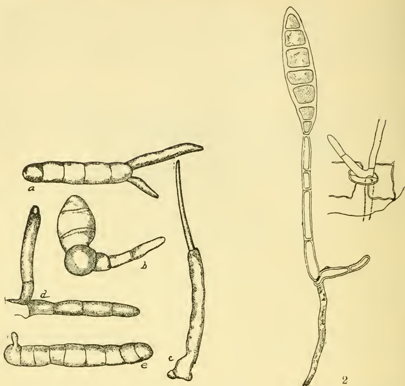
Fig. 101. Spores of Yellow Leaf Disease of Barley ( Helminthosporium graminum ). a. and e. Spores germinating. d. Conidiophore. 2. Leaf browning of Corn ( Helminthosporium turcicum ). Spore and conidiophore to the left. To the right, conidiophore pushing through stoma.
