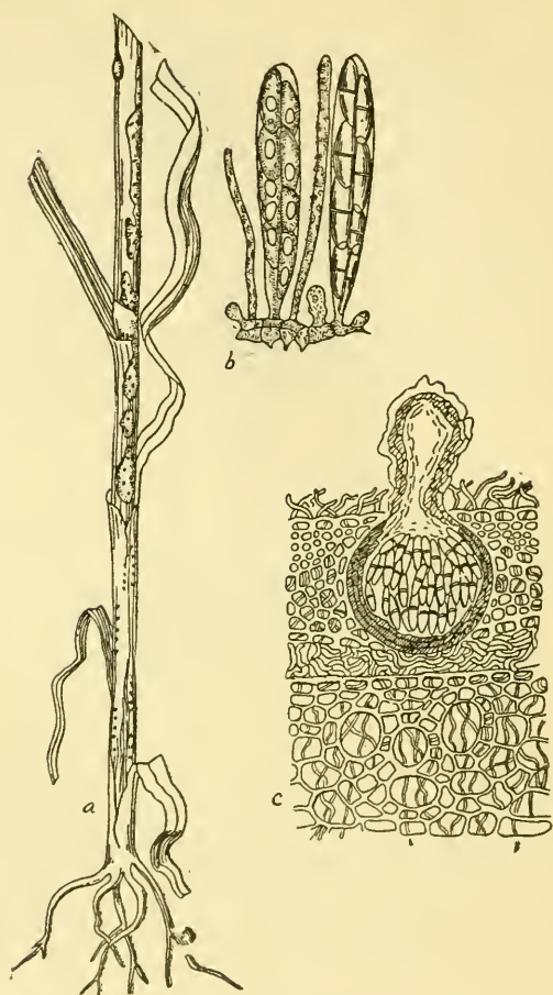
Fig 90. Stem Blight ( Gibberina cerealis ), one of the Sphaeriaceae . a , general appearance. b , asci with ascospores and paraphyses. c , stroma, mycelium, and perithecium. After Cavaia.
