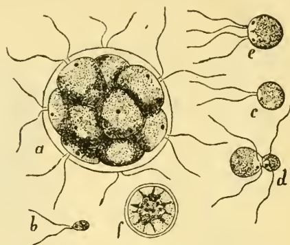
Fig. 34. Chlorophyceae. Pond Scum. Pandorina Morum . a. Floating caenobium. b and c. Zoospores. d. Zoospores conjugating. e. Process of conjugation complete. f. Zygospores. After Luerissen.
