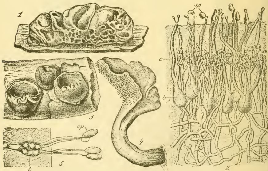
Fig. 59. The Gelatinous Fungi. Tremellineae. 1. Tremella lutescens on wood. 2. Cross section through hymenium, b—Basidia, c—Conidia, sp—Basidiospores, x 450. 3. Exidia truncata . 4. Tremellodon gelatinosum . 5. Basidia of the same x 560. 1-3 after Brefeld. 4-5 after Mueller.
