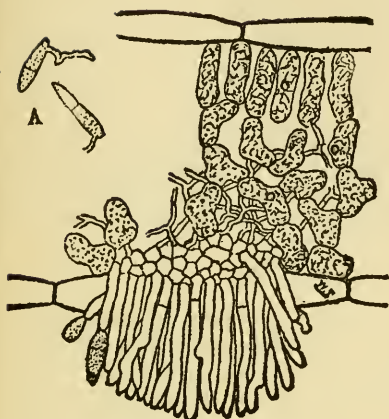
Fig. 101a. Spot Disease of Orchard Grass ( Scolecotrichum graminis ). Cross-section of leaf, general fruiting layer of fungus with conidiophores and conidia. A, spores germinating. After Trelease.
