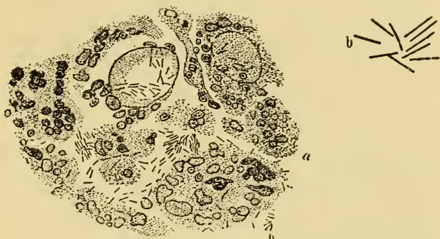
Fig. 30h. Glanders bacillus. a. Section through "glandereal" tissue, the small rods massed or single. b. Bacilli stained with methyl-blue. After Flügge.
