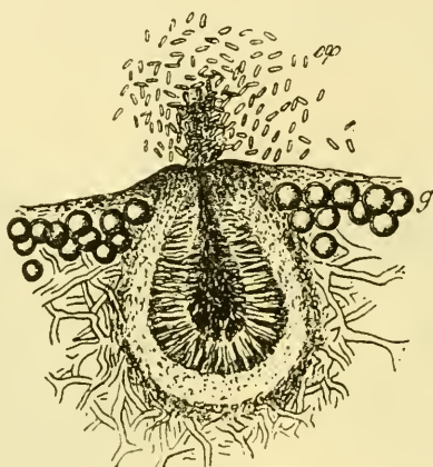
Fig. 114. Spermogonia of Lichen. g. Goniocidia, fungus threads below. sp. Spermatia. Greatly magnified. After Tulacne.
