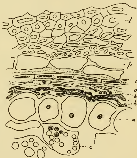
Fig. 153. "Darnel" ( Lolium temulentum ). Section of outer part of a grain which has been in a germinating chamber 24 hrs. l , pale. b , pericarp, i , crushed integuments, o , outer row of nucellus cells, b , cavities with nucellus (probably old cell lumina), h , hyphae, a , aleurone, c , starch endosperm. After Freeman, redrawn by Charlotte M. King.
