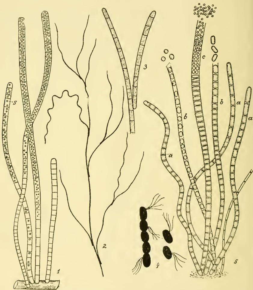
Fig. 25. Chlamydothrixaceae and Beggiatoaceae. 1. Beggiatoa alba , s Sulfur granules x 800. 2-4. Cladothrix dichotoma ; 2 Caenobium x 350. 3. Part of filament magnified 1000 times. 4. Cells with flagellae x 1000. 5. Crenothrix polyspora ; a, young threads; b, threads separating into bodies; c, older threads with spores x 1000. Fig. 1, 2, and 5, after Zopf, Fig. 3 and 4 after Migula.
