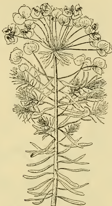
Fig. 337. Yellow Flowering or Cypress Spurge ( Euphorbia Cyarissias ). A branch with large bracts and small flowers. (Strasburger, Noll, Schenck and Schimper.)
