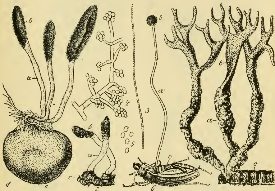
Fig. 95. Various species of Cordyceps . 1. C. ophioglossoides . 2. C. militaris , a Stroma on a caterpillar (c). 3. Stroma on a fruiting form of Elaphomyces granulatus . 4. Conidiophore x 350. 5. Conidia of C. ophioglossoides . 6. C. cinerea on a beetle (c). 7. C. Taylori on a caterpillar (c). a in all figures sterile, b fertile part of the Stroma. 1 and 6 after Lindau. 3-5 after Brefeld.
