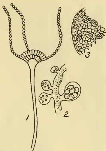
Fig. 89a. Aspergillus nidulans . 1. Conidiophore. 2. Branch of mycelium with asci and ascospores, magnified. 3. Asci. Cross section. Ascus. All greatly magnified. (After Eidam.).
