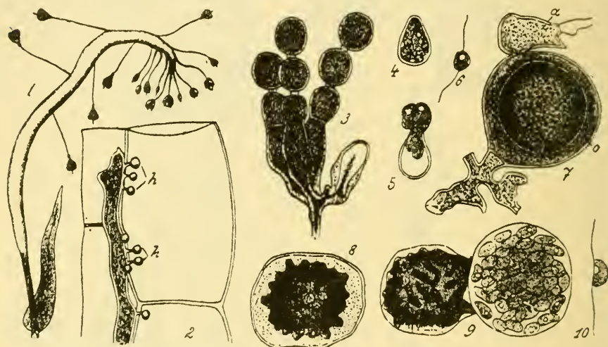
Fig. 48. Peronosporaceae. White Rust. Albugo canida . 1. Inflorescence of Shepherd's Purse with fungus. 2. Mycelium with haustoria (h) x 390. 3. Conidiophores and conidia (spores) in chains x 400. 4 and 5. Formation of zoospores in conidia x 400. 7. Oogonium (o) and antheridium (a) attached, mycelium shown below. 8. Oospore with thick wall. 9. Germinating oospore forming a zoosporangium. 10. Zoospore. 7-10x400. 6. Germinating Zoospore. After DeBary.
