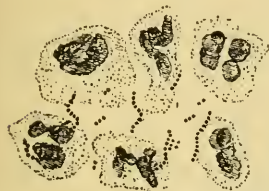
Fig. 28. Pus organism. been held by some authors to cause rheumatic fevers Streptococcus pyogenes . In Af. and also scarlet fever. Probably many so-called terminal infections are produced by this organism.
