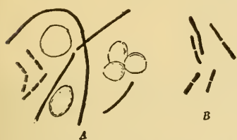
Fig. 30b. Malignant Oedema. Bacillus oedematis maligni . A. From spleen of guinea pig. B. From lung of mouse. Both x 700. After Koch.
