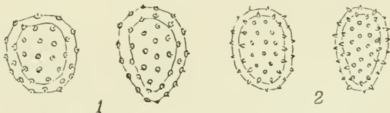
Abbild. 3. Phragmidium Rubi Idaei . 1 Caemasporen, 2 Uredosporen. \frac{824}{1}
