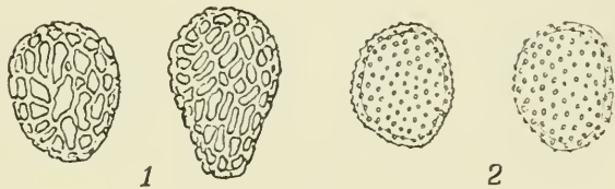
Abb. 1. Phragmidium Rubi . 1 Caemasporen, 2 Uredosporen. \frac{824}{1}
