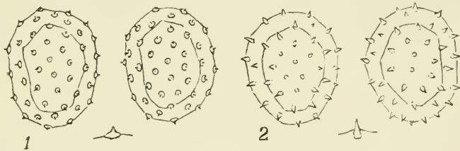
Abbild. 2. Phragmidium violaceum . 1 Caemasporen, 2 Uredosporen. \frac{824}{1}
