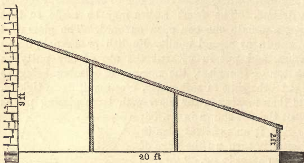
Fig. 60.—LEAN-TO GRAPERY.
