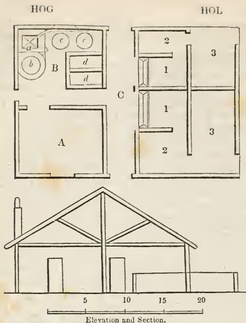
Elevation and Section.
