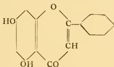
Quercetin , or tetrahydroxy-flavonol *
