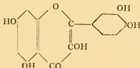
Quercetin , or tetrahydroxy-flavonol *
