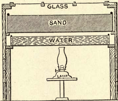
48. Simple propagating-oven.
