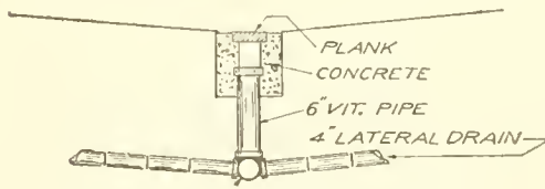
1360. Detail of drain connections. (See Fig. 1356.)
