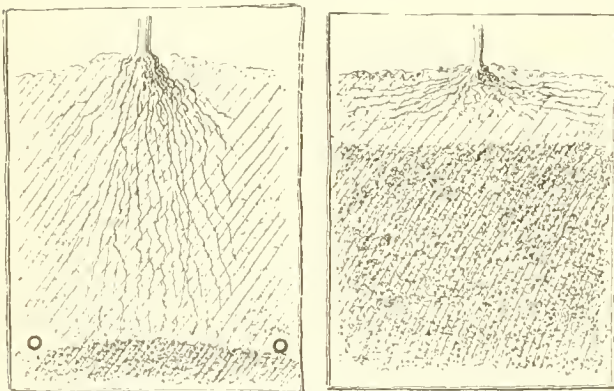
1347. Diagrams to explain the effect of lowering the water-table by means of under-draining. On the undrained soil, the roots do not penetrate deep; and when droughts come, the plants suffer.
