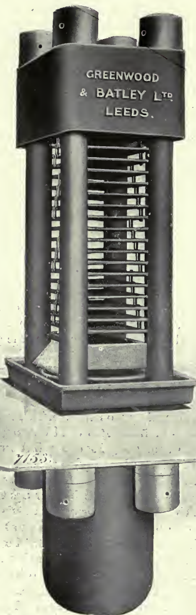
ANGLO-AMERICAN HYDRAULIC OIL PRESS
