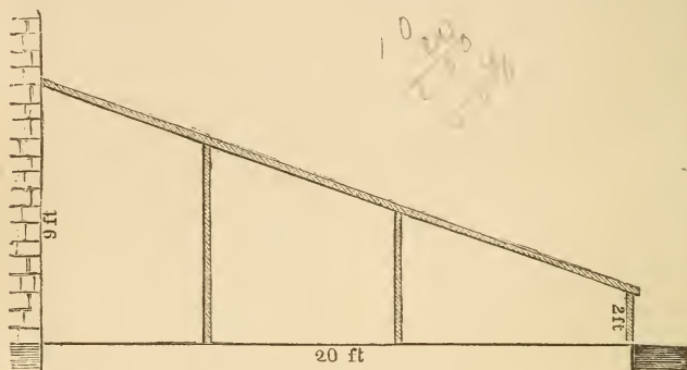
Fig. 60.—LEAN-TO GRAPERY.
