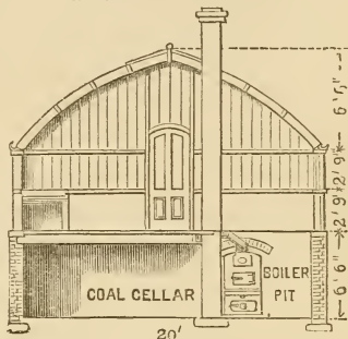
Fig. 44.—END-VIEW OF FIG. 43, AT BOILER PIT.
